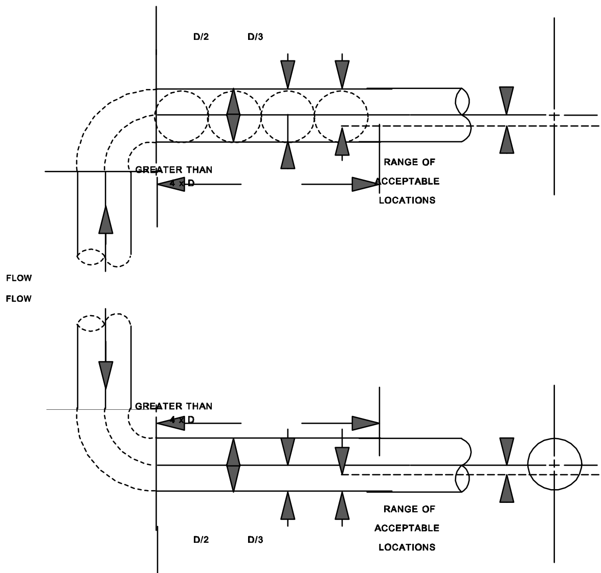
Figure 1-4. Transmissometer location greater than four diameters downstream of a vertical bend in a horizontal stack or duct.
