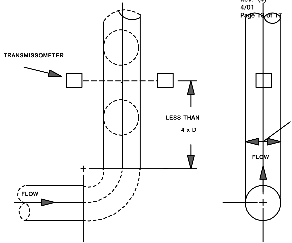
Figure 1-1. Transmissometer location downstream of a bend in a vert
