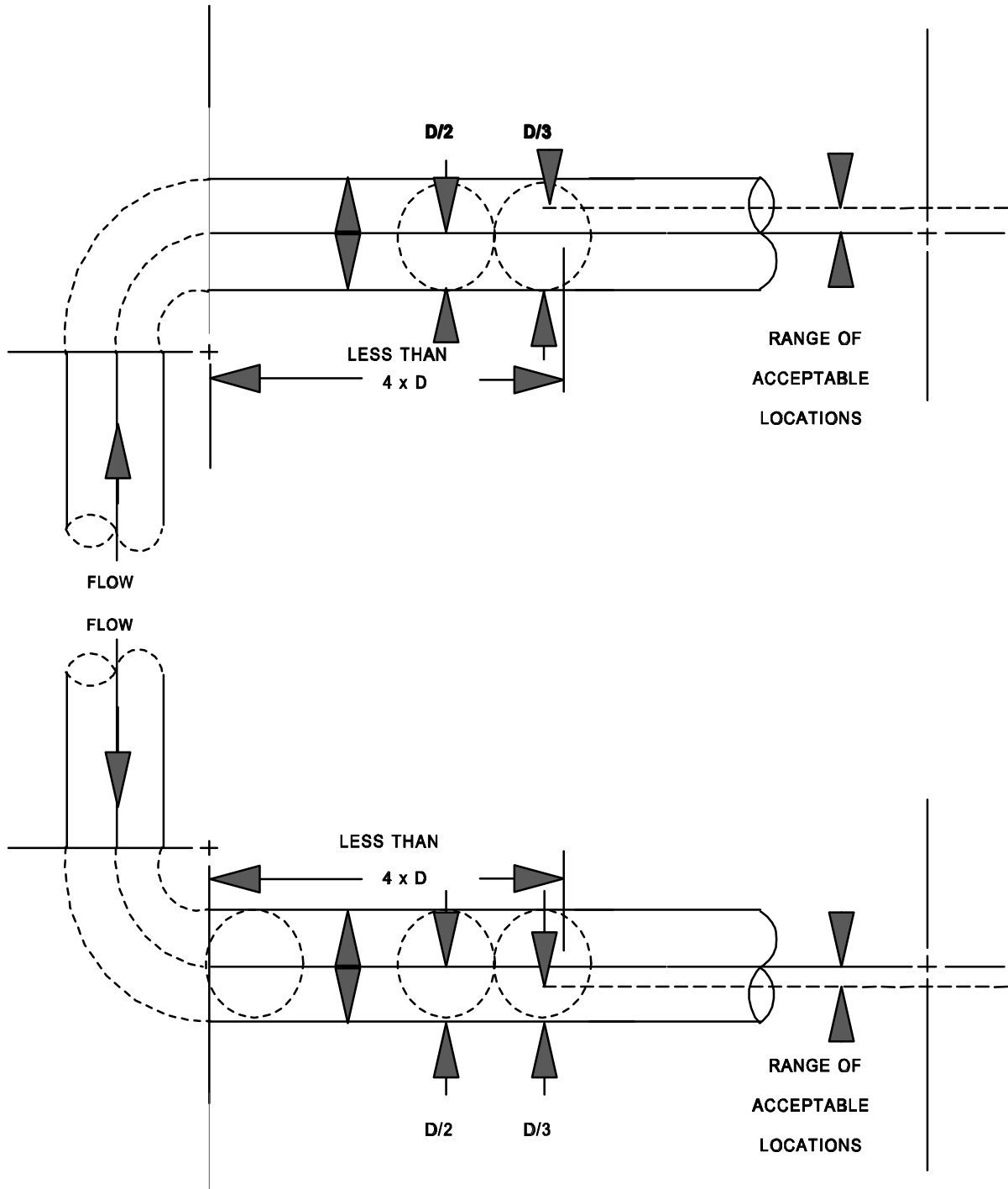
Figure 1-5. Transmissometer location less than four diameters downstream of a vertical bend in a horizontal stack or duct.
